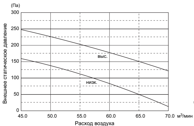
PEA-RP200GA
