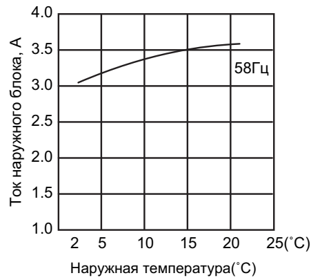
SUZ-KA35VA(H).TH
