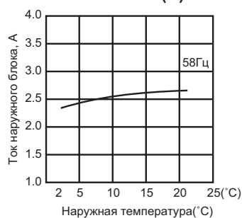
SUZ-KA25VA(H).TH
